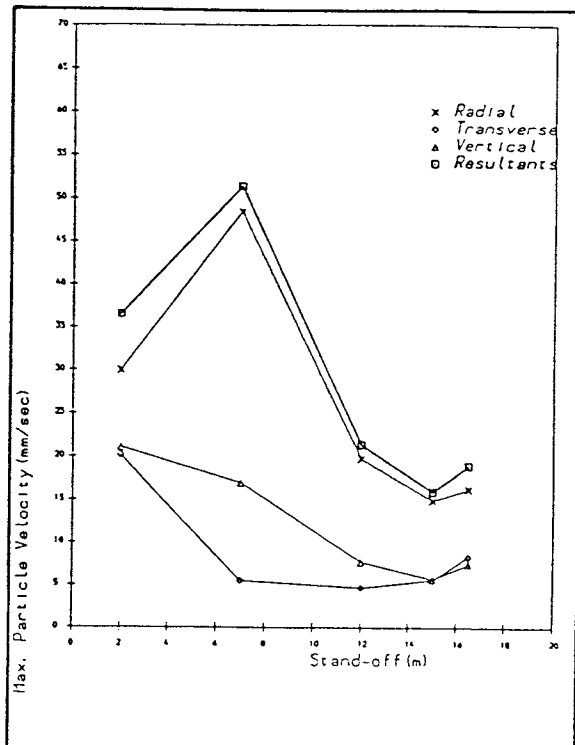
Figure 8. Attenuation of vibrations - drop hammer
