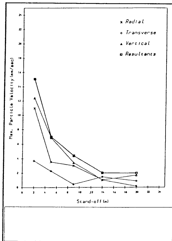
Figure 6. Attenuation of vibrations with distance - vibrodriver
